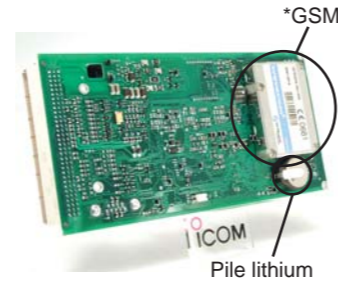
Pile lithium
